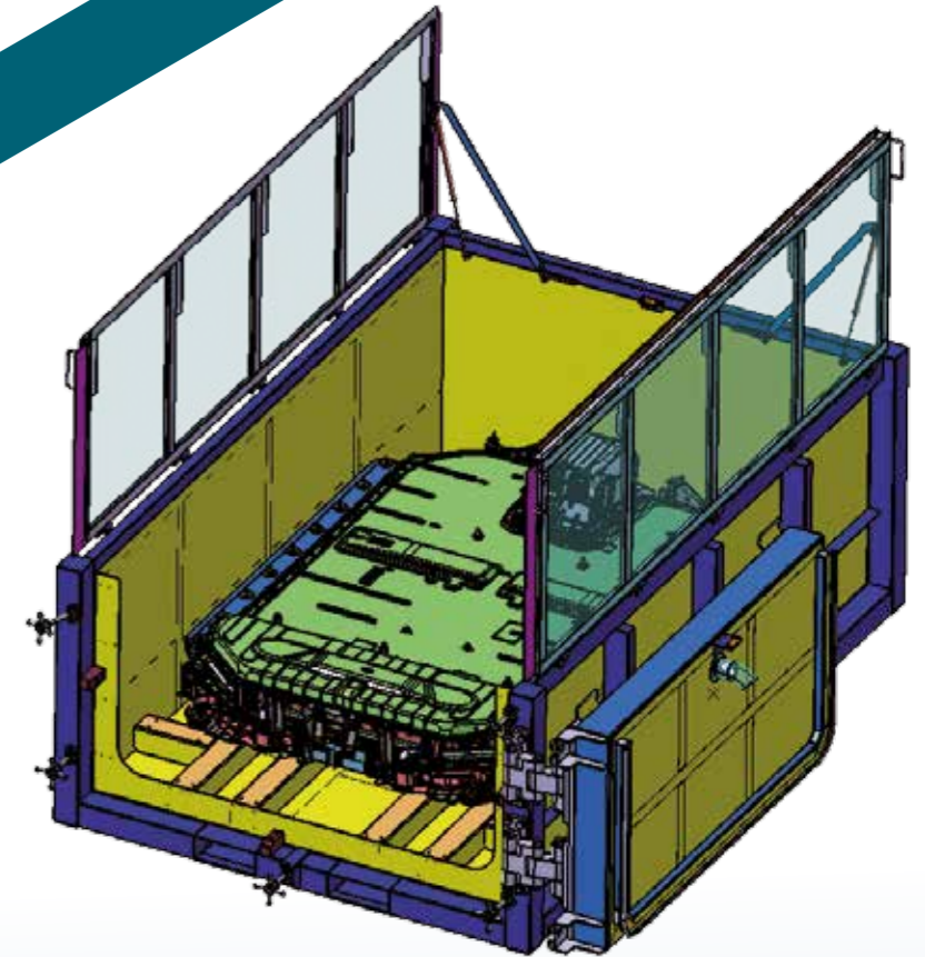
Emergency container with battery unit
